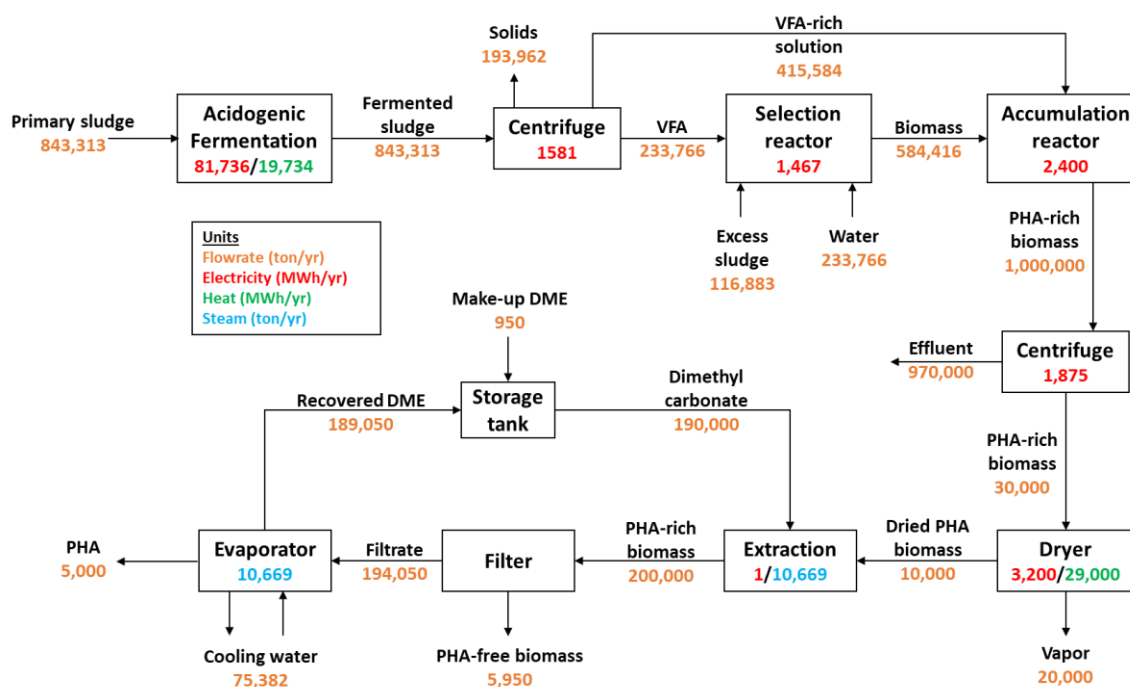
Figure 5. Mass and energy balance of PHA production
